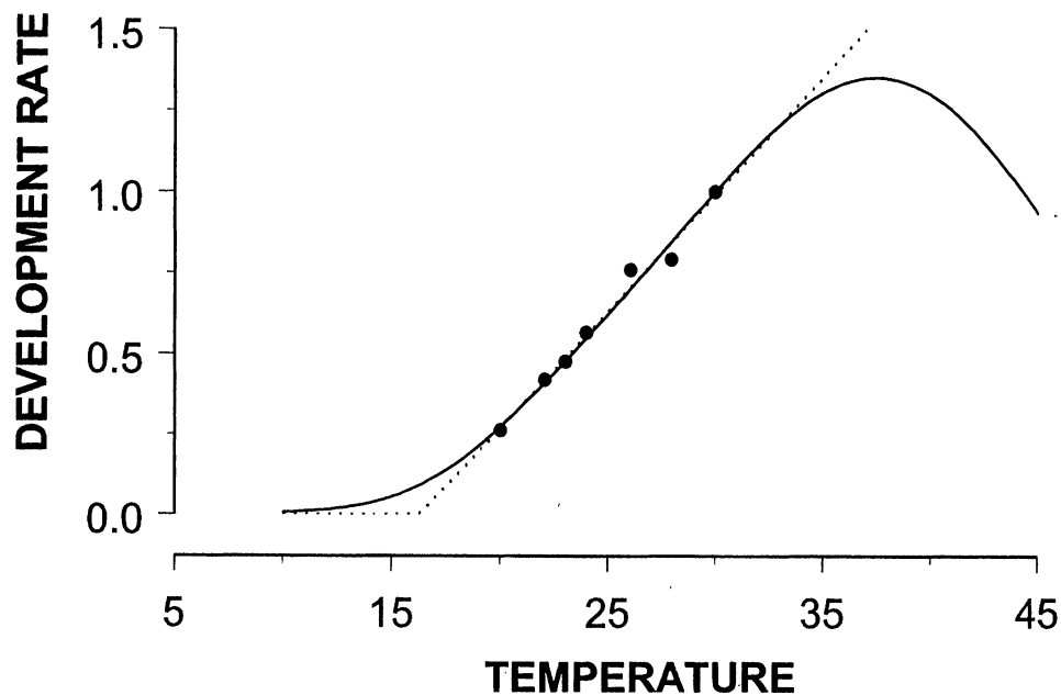
Figure 9.2 The Sharpe-DeMichelle model (solid line) and linear degree-hours model (broken line) applied to developmental rates of the temperate-zone lizard Bassiana duperreyi . Data are calculated from Figure 2 of Shine and Harlow (1996). Development rate is incremental change in head width, expressed as a percentage of final hatchling head width, per day. The linear model was fitted by least squares regression ( ds/dt = 0.07251 T - 1.1818 ). The Sharpe-DeMichelle model was optimized at lower temperatures using development rates for 23.0 \pm 3.75^\circ\text{C} and 23.0 \pm 9.75^\circ\text{C} (Shine and Harlow 1996). The curvature at higher temperatures is not supported by data and is shown for illustration only. Parameters of the Sharpe-DeMichelle curve are RHO_{25} = 0.7 , H_A = 17199.9 , T_L = 291.47 , T_H = 311.71 , H_L = -64401 , and H_H = 41965 . Note the close agreement between the linear model and the Sharpe-DeMichelle model at intermediate temperatures.
