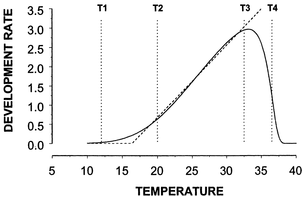
Figure 9.3 The Dallwitz-Higgins model (1992) (solid line) and the linear degree-hours model (broken line) applied to hypothetical data. Developmental rate is incremental change in head width, expressed as a percentage of final hatchling head width, per day. Note the close agreement between the linear model and the Dallwitz-Higgins model at intermediate temperatures, similar to that of the Sharpe-DeMichelle model of Figure 9.2. T_1 and T_4 are the lower and upper absolute lethal limits, outside which even brief exposure causes embryo death or gross abnormality. T_2 and T_3 are the constant-temperature lethal limits, outside which a temperature held constant throughout incubation will cause embryo death or gross abnormality. Temperatures in the sublethal ranges T_1 - T_2 and T_3 - T_4 will support embryonic development, provided exposure is for a part of each day only, but the duration of exposure that can be tolerated will decline as one moves to extremes.
